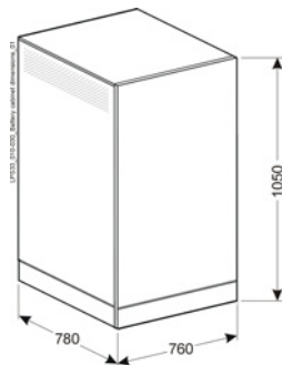
Battery cabinet
